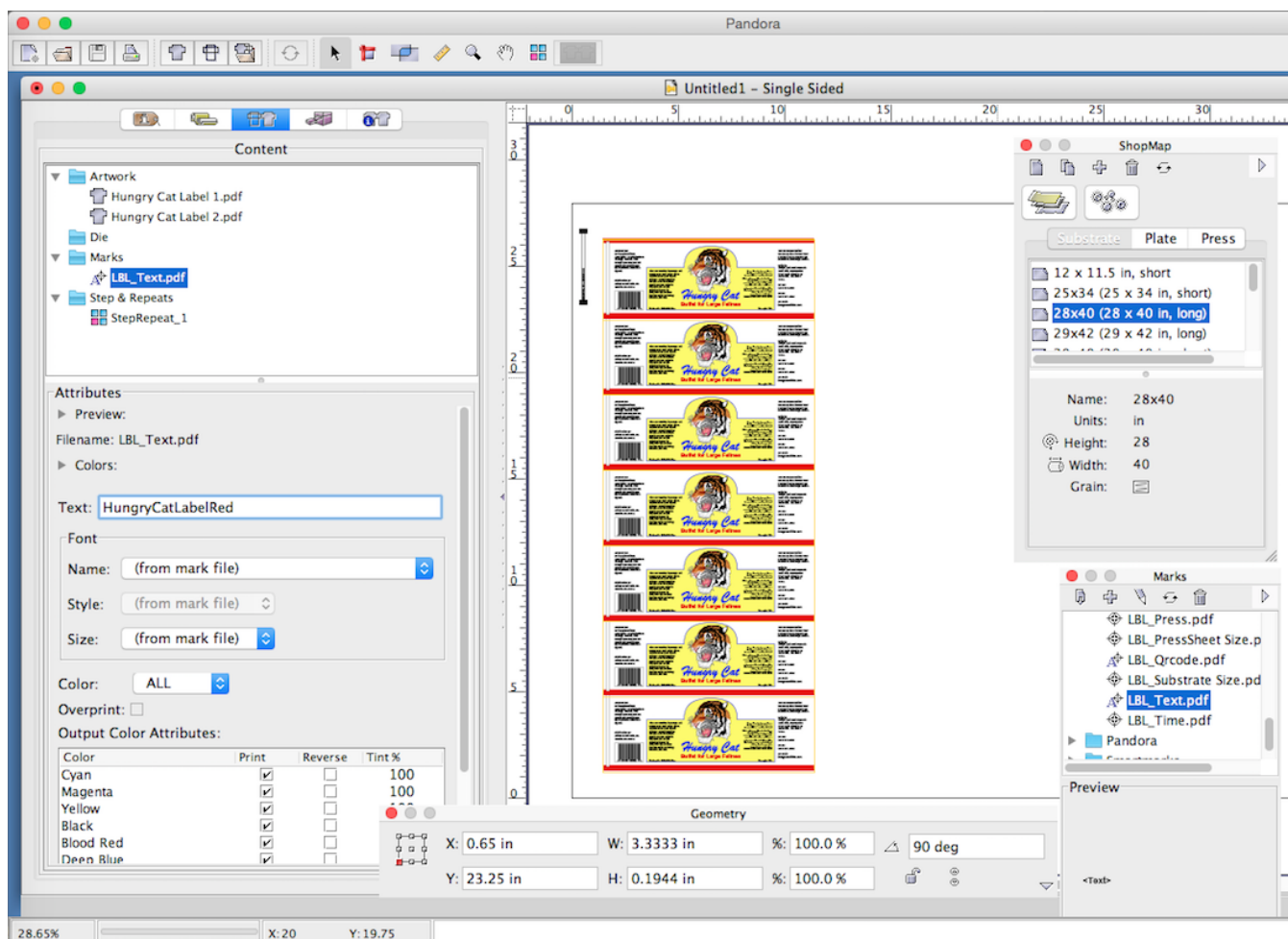
Figure 1. Job window
