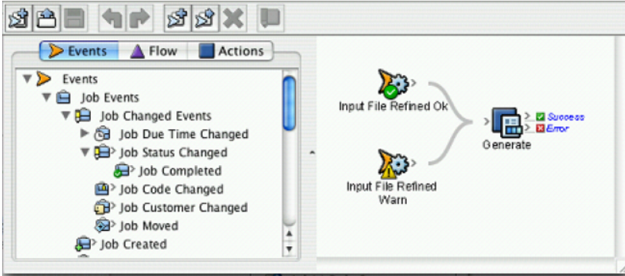
Rule to Generate After Refine
