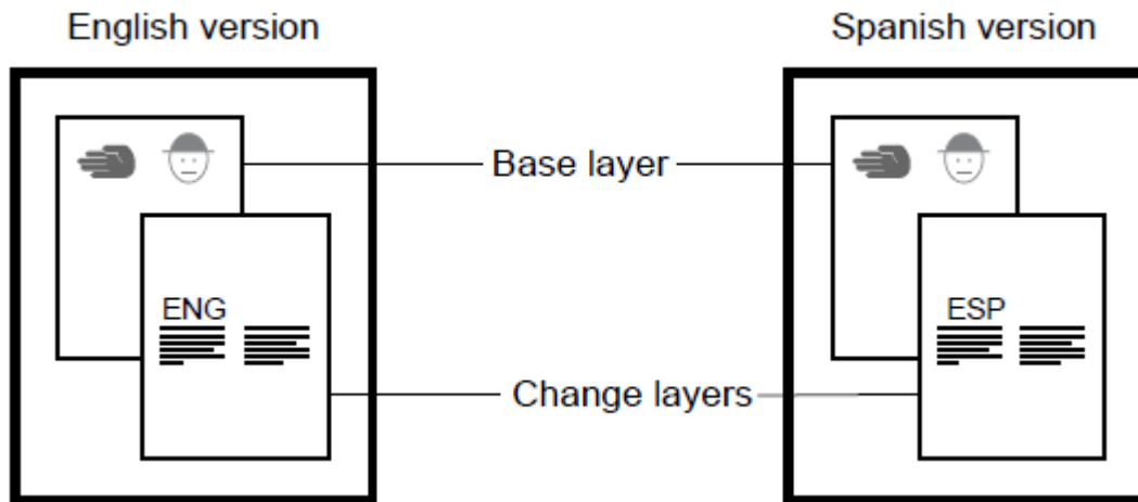
Figure 1. Versions and layers
